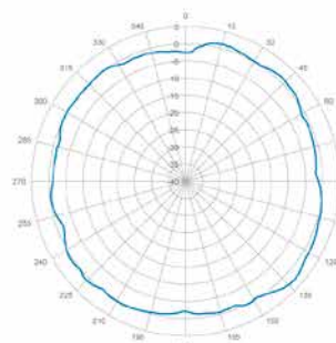
5 GHz Elevation
