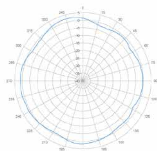
2.4 GHz Azimuth
