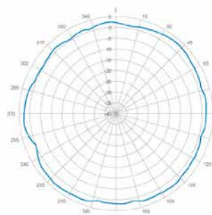
5 GHz Azimuth
